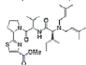
aeruginosamide ( C_{20}H_{31}N_5O_2 ) (88-7, CHCl_3 )
